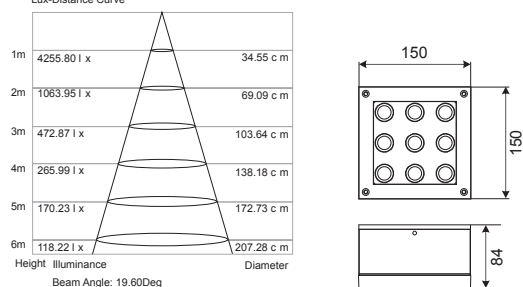
Lux-Distance Curve
