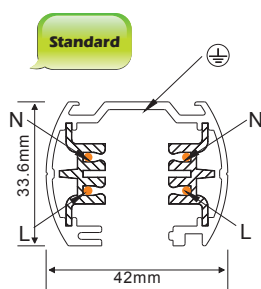
3-Wire Single Circuit Track
