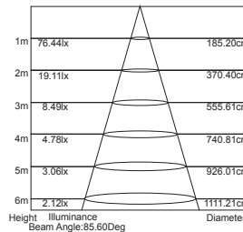
Lux-Distance Curve
