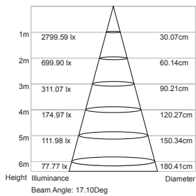
Lux-Distance Curve
