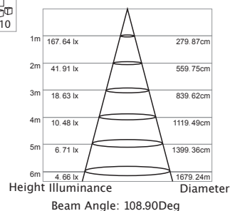
Lux-Distance Curve
