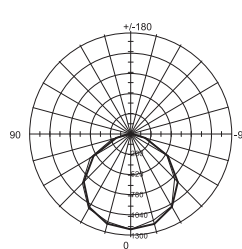
Light Distribution Curve[Unit.cd]
