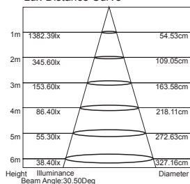
Lux-Distance Curve
