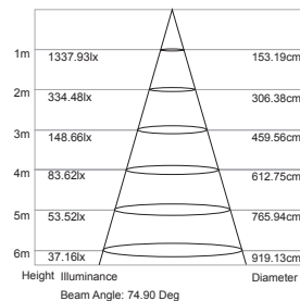
Lux-Distance Curve
