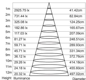
Lux-Distance Curve
