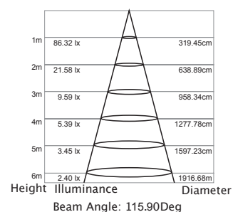
Lux-Distance Curve
