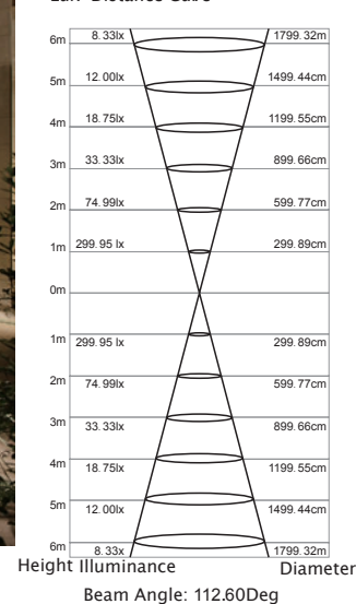
Lux-Distance Curve
