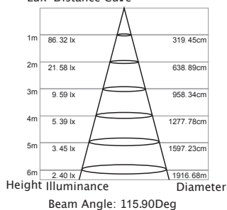
Lux-Distance Curve
