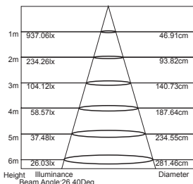
Lux-Distance Curve
