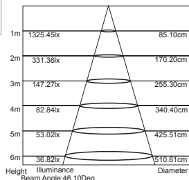
Lux-Distance Curve
