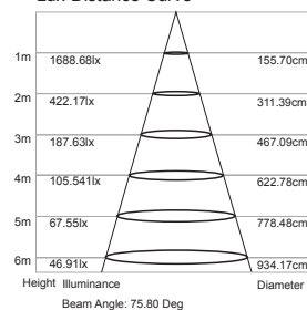
Lux-Distance Curve
