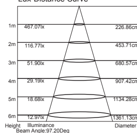
Lux-Distance Curve
