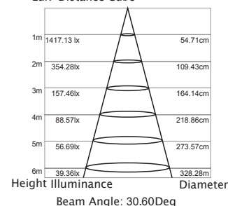
Lux-Distance Curve
