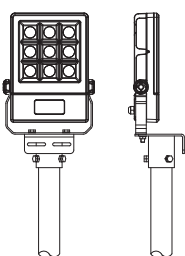
Installation Drawing 2
