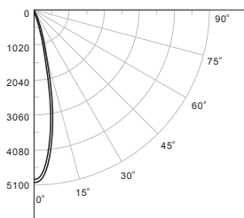
Lux-Distance Curve
